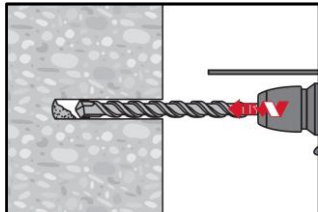
Hammer drill
